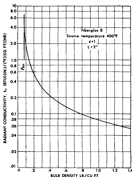
Fig. 17. Effect of bulk density on radiant conductivity of Fiberglas B.
