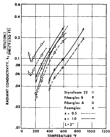
Fig. 16. Effect of temperature on radiant conductivity.
